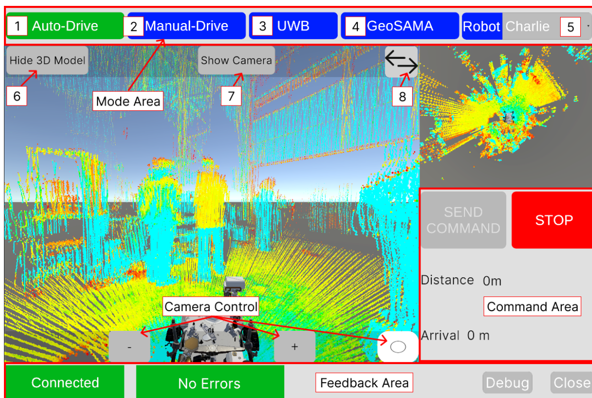
Figure 4.2: The User Interface when starting the application, showing the point cloud produced by the laser scanner from the Robot “Charlie”.
