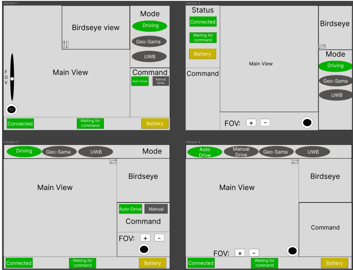
Figure 4.1: The four designed low-fidelity prototypes, differ in the arrangement and scale of the areas.
