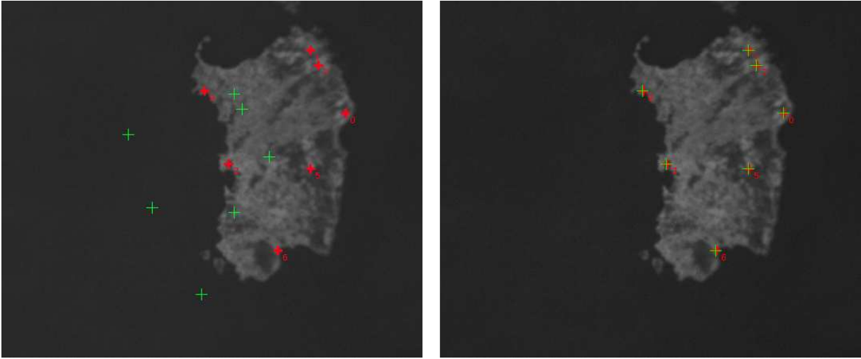
Figure 2.3: IBVS: A simulation of an attitude control on an orbiting satellite based on the actual tracked features (red) and the desired features (green).
