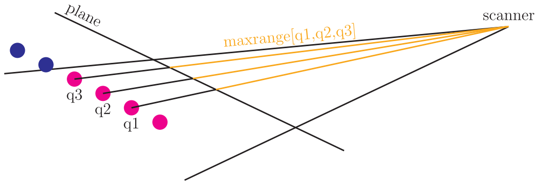
Fig. 13. The plane is also used to cap the search distance up to the angular range neighbors of p . The neighbors of p are q1 , q2 and q3 marked in magenta and the maximum search distance marked in orange. (For interpretation of the references to color in this figure legend, the reader is referred to the web version of this article.)
