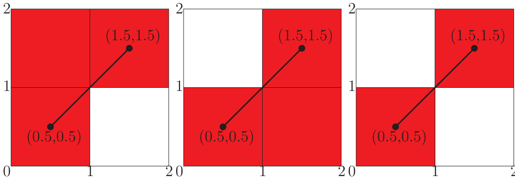
horizontal dimension first, then voxel (1,0) is added to the result. Right: Our algorithm only traverses voxel (0,0) and voxel (1,1). (For interpretation of the references to color in this figure legend, the reader is referred to the web version of this article.)
