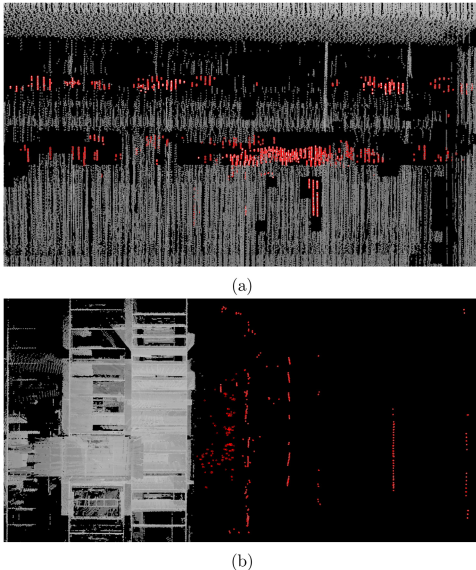
Fig. 31. The high reflectivity of surfaces commonly found in factory environments poses a great challenge. The wall in the top figure has holes because of reflected points “behind” the wall (in red). These points are false as the wall is solid and the area on the right in the bottom figure should be empty. Top: “Holes” in the wall created by points (in red) recorded behind the wall. The points are not exactly aligned with the holes due to parallax. Bottom: Top-view of the scene, showing the same points behind the wall (in red). (For interpretation of the references to color in this figure legend, the reader is referred to the web version of this article.)
